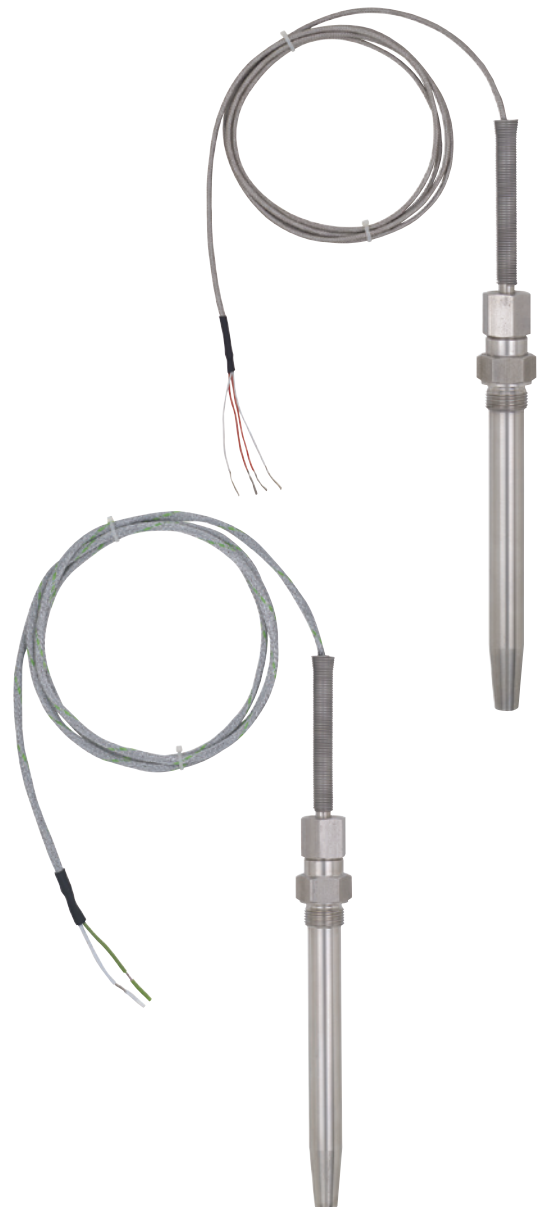
Fig. above: Cable Resistance Thermometer Model TR192 Fig. below: Cable Thermocouple Model TC192
